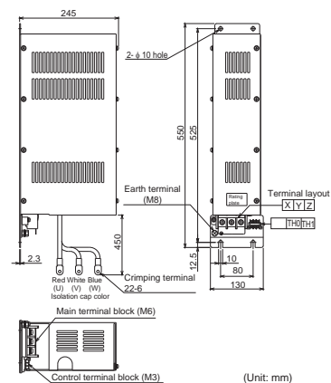
FR-BMF-H37K
