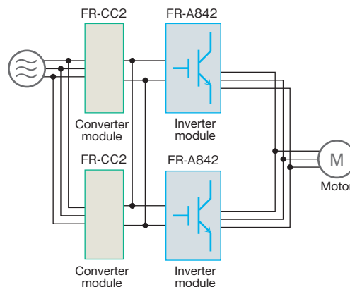
Parallel driving
