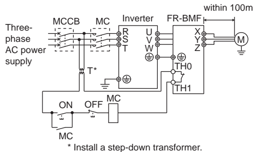
FR-BMF-H7.5K
