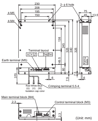
FR-BMF-H7.5K
