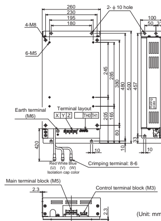
FR-BMF-H15K, H22K
